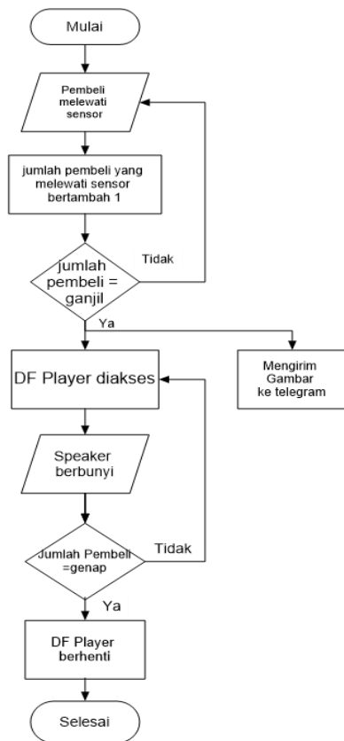
Gambar 3.3 Flowchart Sistem
